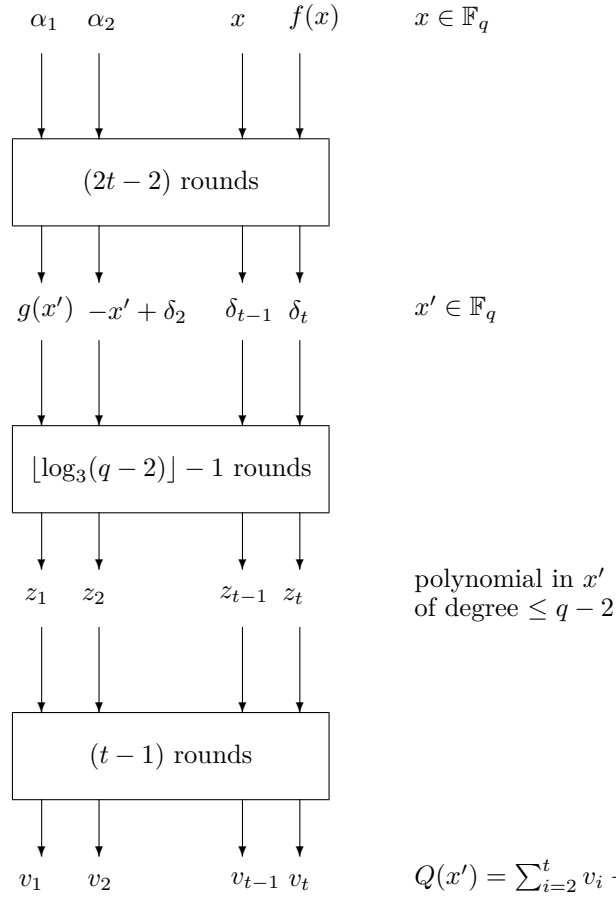
Figure 4: Integral distinguisher on GMIMC.
