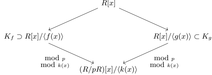
Fig. 1: Commutative diagram of exTNFS. When R = \mathbb{Z} this is the diagram of NFS for non-prime fields. When k(x) = x - m for some m \in R this is the diagram of TNFS. When both R = \mathbb{Z} and k(x) = x - m this is the diagram of NFS.
